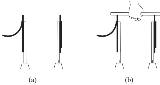
Figure 6.32: (a) Electroscoposcope I is charged. (b) A neutral straw is then placed in such a way as to connect both electroscopes. Nothing changes when this is done.
