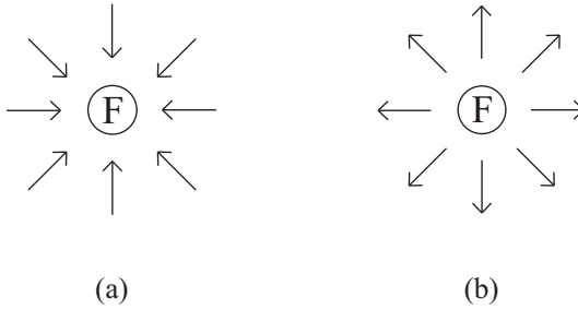
Figure 4.33: (a) Before contact the arrows point toward the rubbed straw, being attracted by it. (b) After contact they point away from the plastic, being repelled by it.
