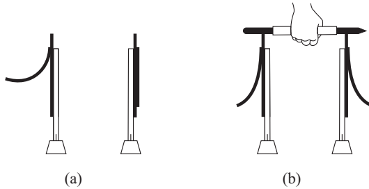
Figure 6.33: (a) Only electroscoposcope I is charged. (b) A wood skewer is surrounded by a plastic straw, with the wood supported by the two electroscopes. We observe that strip I falls a little, while strip II rises a little.
